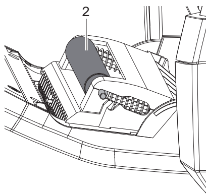
Pressure roller in working position
