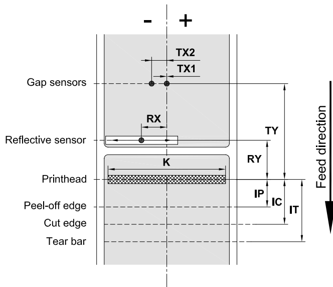
Figure 24 Device dimensions
