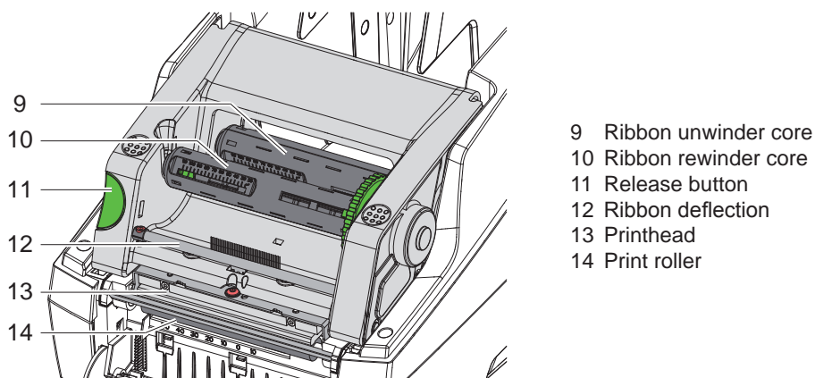
Figure 2 Print module
