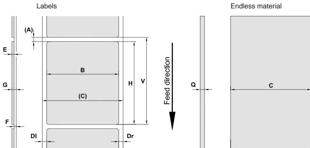
Figure 23 Label / endless material dimensions
